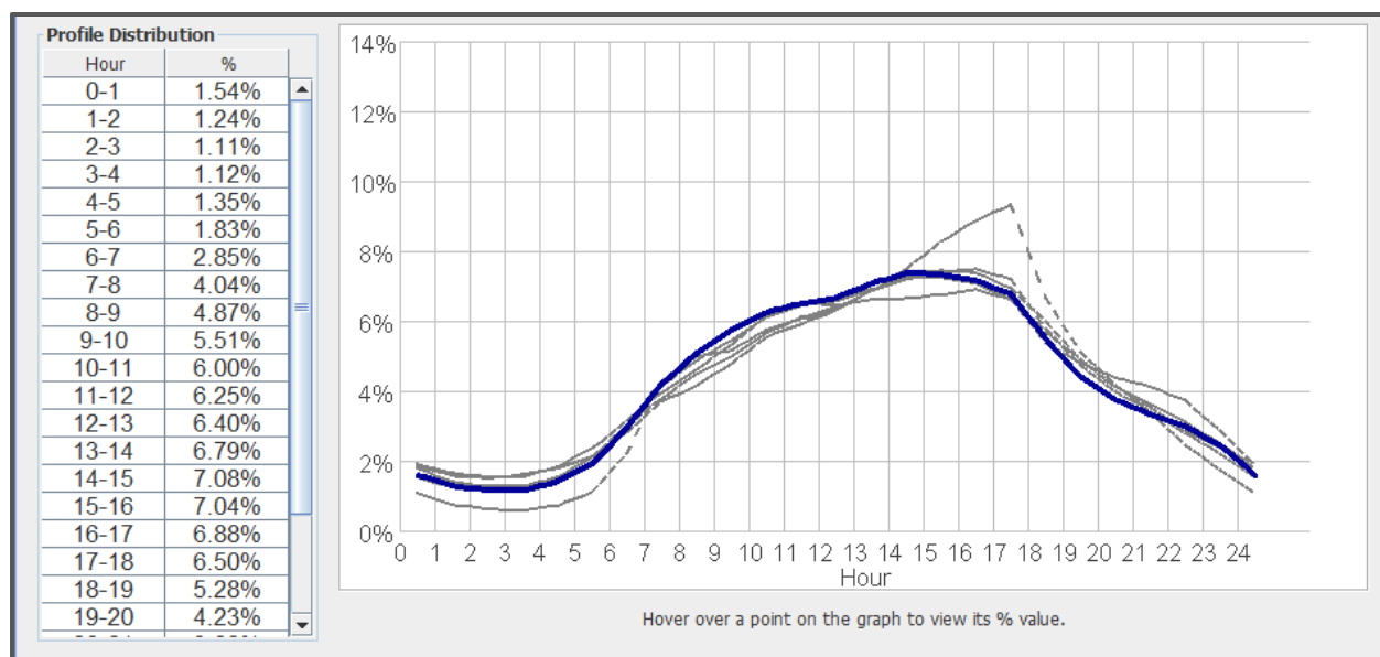
Figure 10: Unimodal AADT Distribution Shape.
