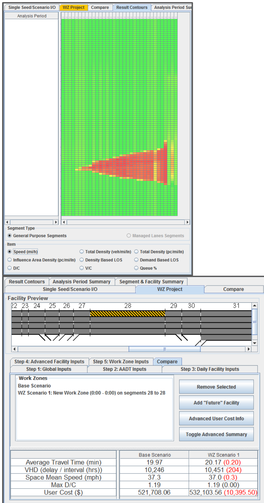
Figure 7: Analysis with a study period from midnight to midnight which completely contains the congestion dynamics.
