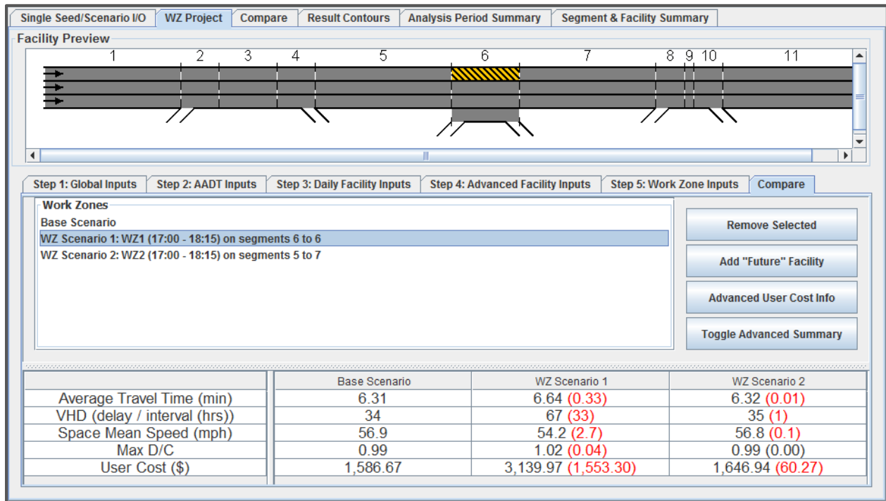
Figure 34: Comparison analysis of the two work zones.
