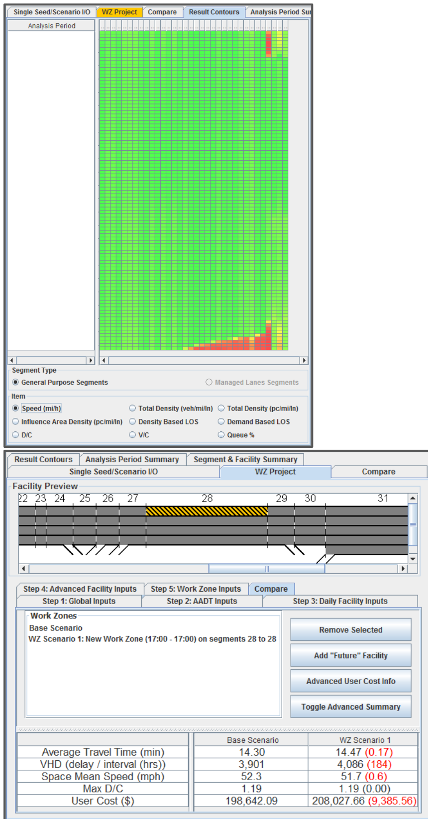
Figure 8: Analysis with a study period from 17:00 to 17:00 which fails to properly contain the congestion dynamics.
