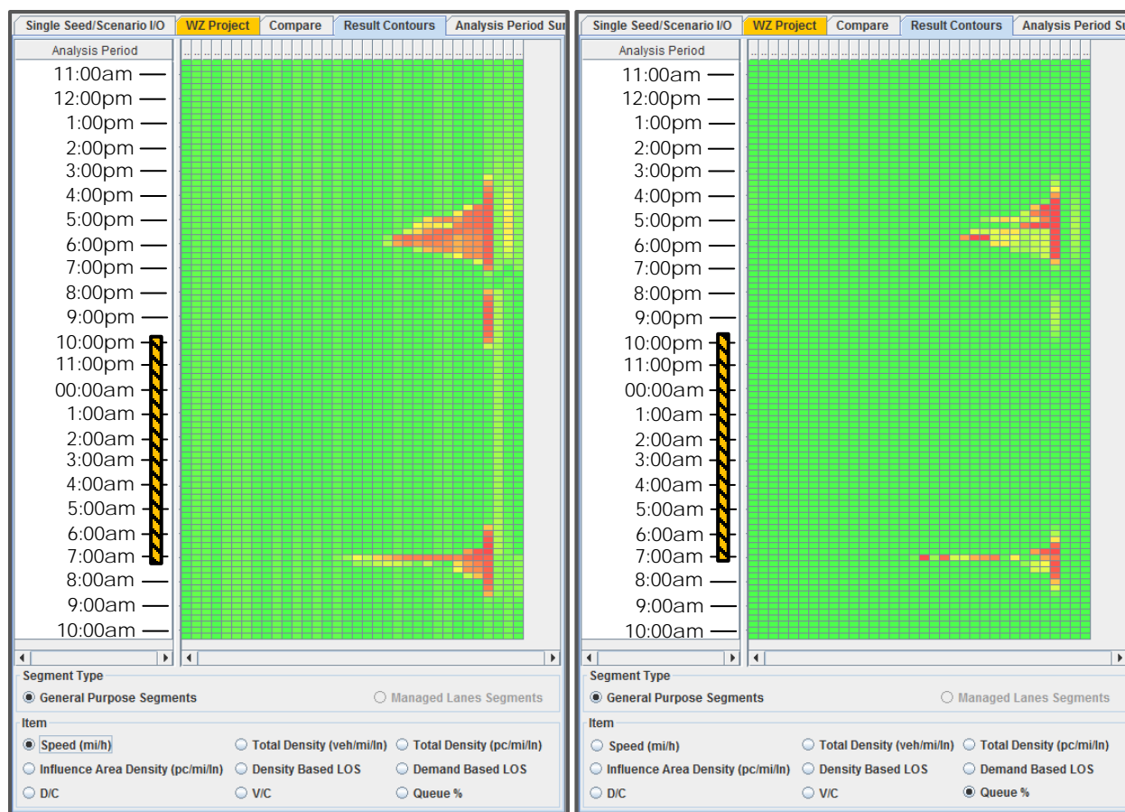
Figure 6: Contour plots for speed and queue % showing that the areas of congestion are fully contained within the 24 hour study period which runs from 10:30am – 10:30am.
